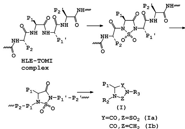
Figure 1. Evolution of the design of inhibitor (I) beginning with the human leukocyte elastase–turkey ovomucoid inhibitor (HLE–TOMI) complex.
