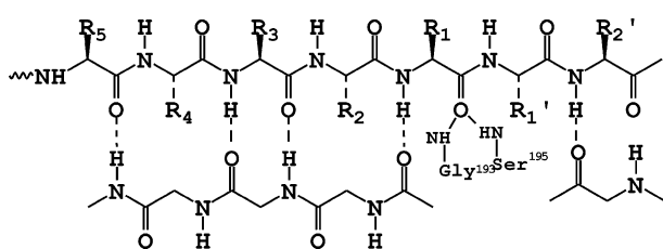
Figure 3. Main-chain and side-chain binding interactions between a substrate or inhibitor and the active site of HLE.
