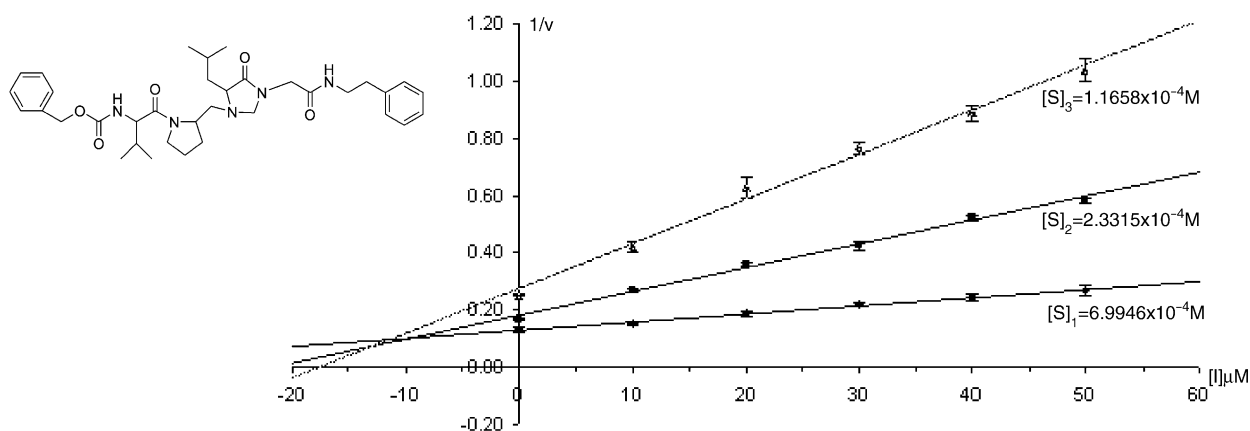
Figure 2. Dixon plot showing the inhibition of human leukocyte elastase by compound 11 .
